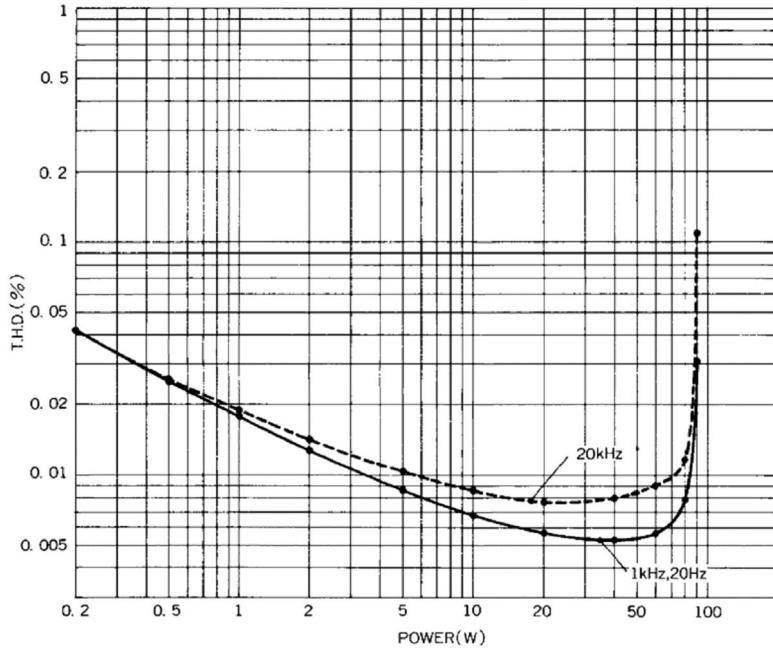
L-55A T. H. D. VS POWER (INPUT:AUX, OUTPUT:SP, TONE:FLAT, 8Ω LOAD BOTH CH, DRIVEN)
