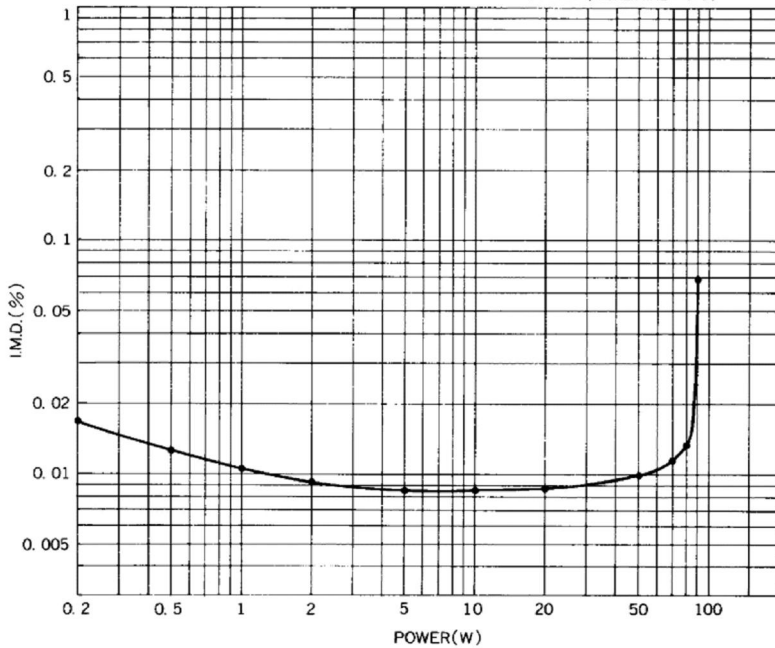
L-55A I. M. D. VS POWER (INPUT:AUX, OUTPUT:SP, TONE:FLAT, 8Ω LOAD BOTH CH, DRIVEN, 60Hz, 7kHz=4:1)
