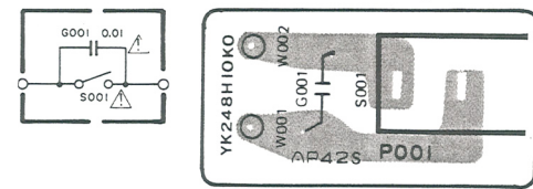
12.6 Power Switch Assembly (PO01) Schematic Diagram and Component Locations
