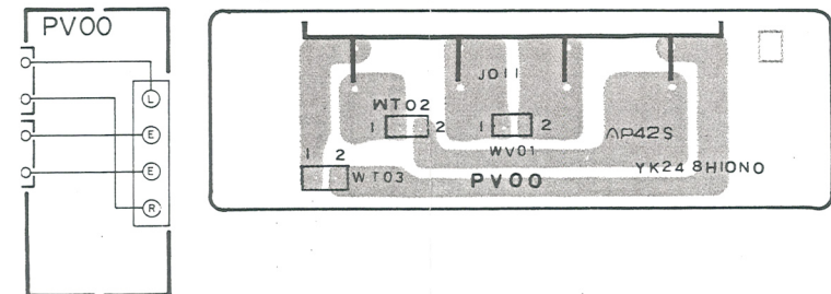
12.7 Speaker Terminal Assembly (PV00) Schematic Diagram and Component Locations
